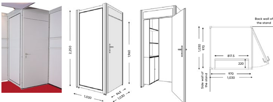
Cubicle 1 m × 1 m, with door and cabinet unit back left, € 1,468
