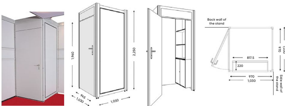
Cubicle 1 m × 1 m, with door and cabinet unit back right, € 1,468
